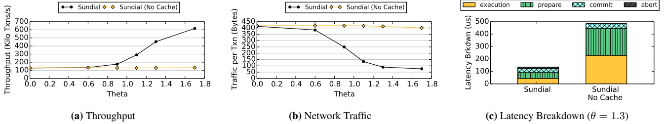
Figure 10: Caching with Read-Write Tables – Performance of Sundial with and without caching on YCSB as the skew factor of read distribution changes.
